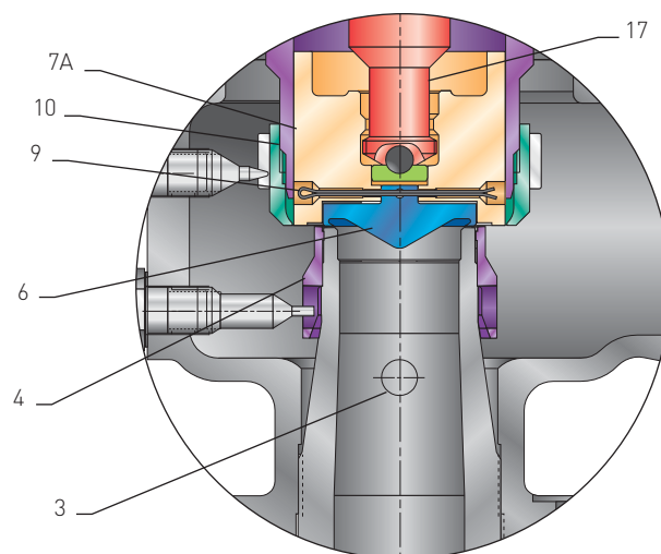
K - Q ORIFICE CONSTRUCTION
